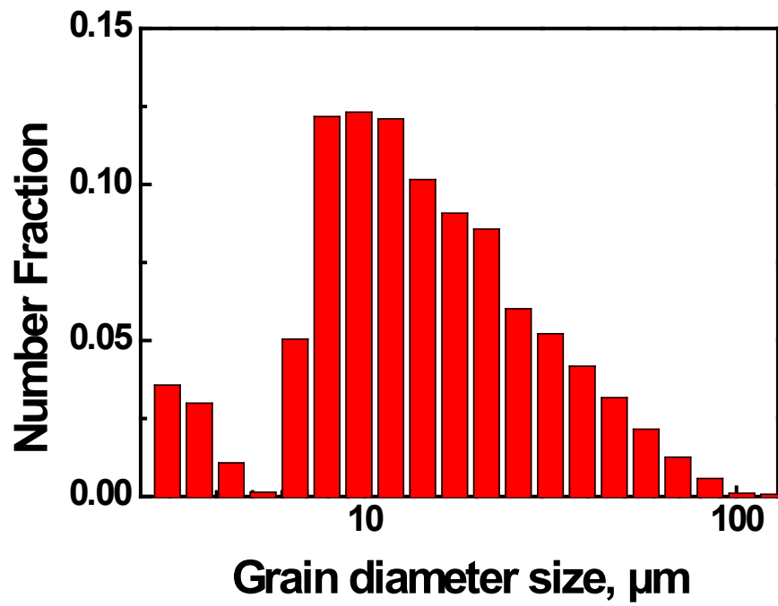
Supplementary Figure S1. Grain size distribution of the LPBF sample on the Z plane.
